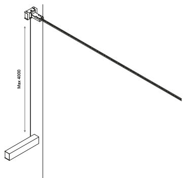
FLASH and INFINITO: example of installation with wall/ceiling driver
