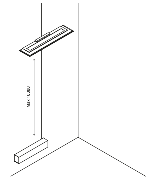
REFLEX: example of installation with wall/ceiling driver
