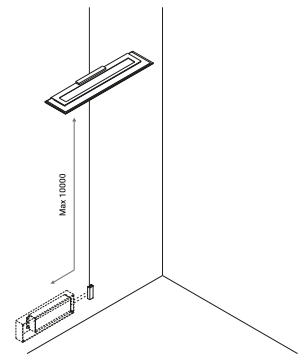
REFLEX: example of installation with remote driver
