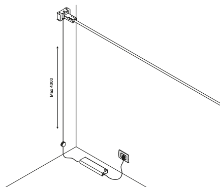
Example of installation with driver with plug
