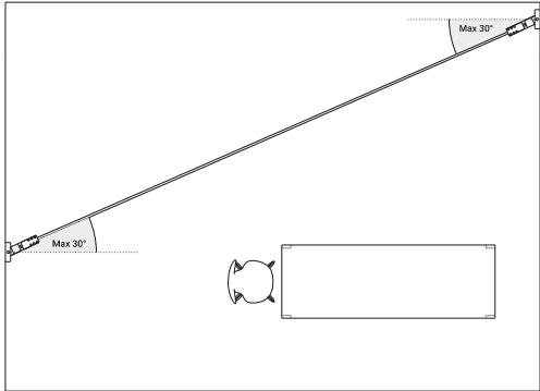
Example of installation with max rotation 30°
