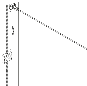
Example of installation with remote driver
