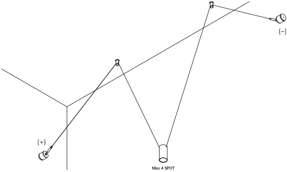
Suspension version
